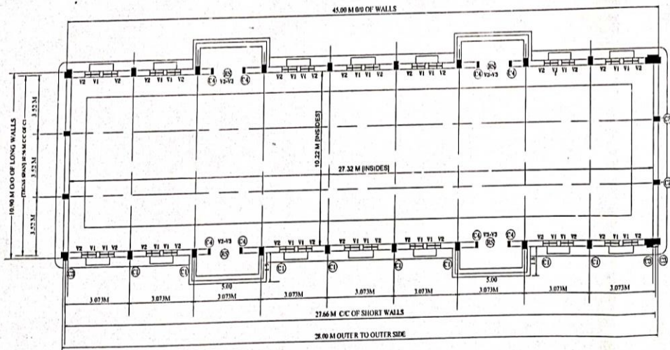
PLAN FOR 460 MT. WAREHOUSE UNIT NO. I, II
